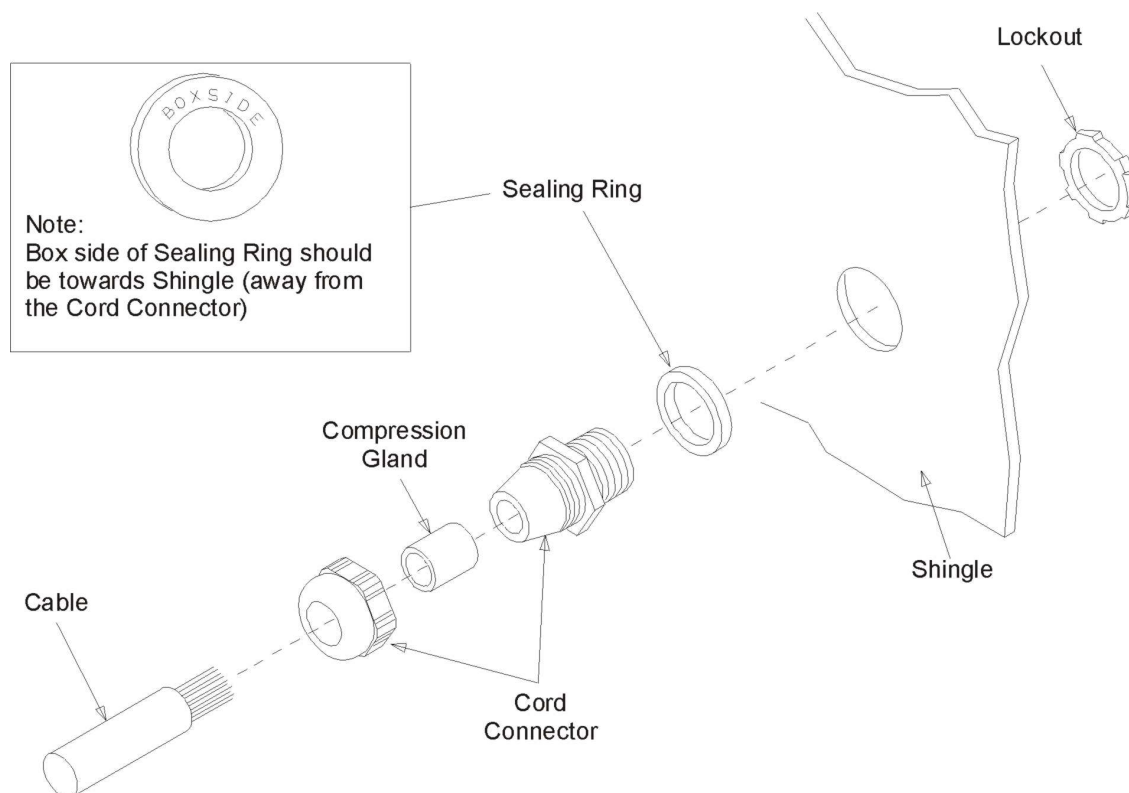
Figure 1. D-Kit Parts
