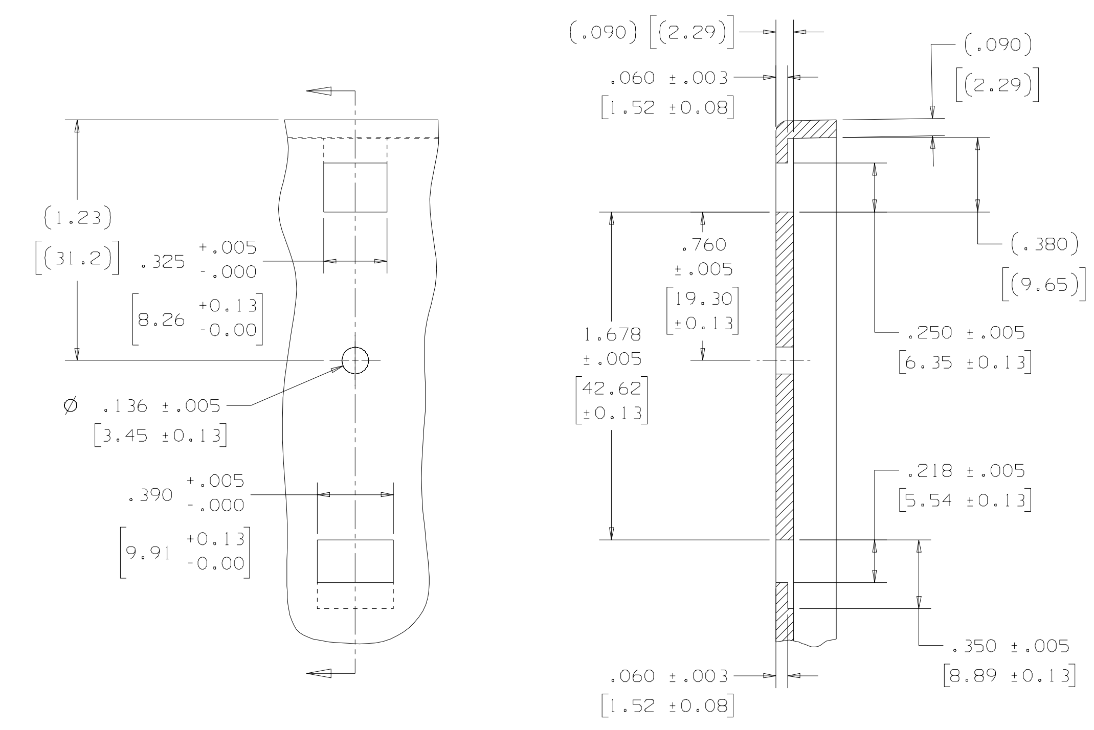
DETAIL A SCALE 2/1 (TYP 6 PLACES MARKED "A")
