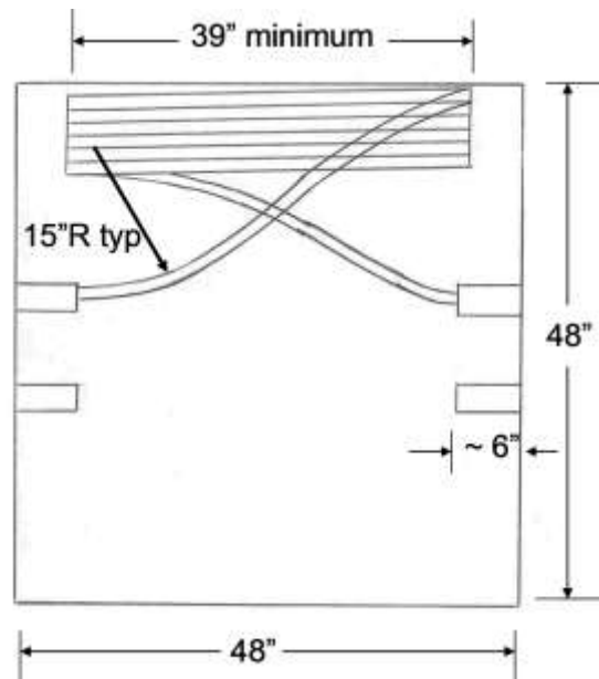
Figure 3 – Cable routing in 48" x 48" manhole (top view).
