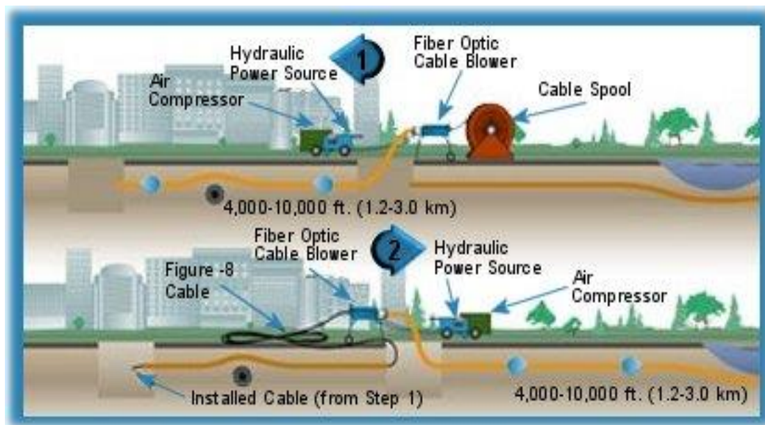
Figure 11 - Backfeed installation using cable blowing equipment.
