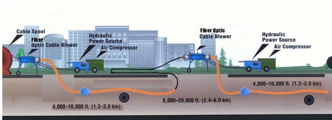
Figure 12 – Forward-feed installation using two cable blowers.
