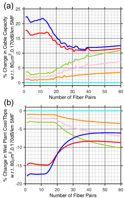
Figure 2: Advanced fibers compared to 80\mu\text{m}^2 , 0.170 dB/km fiber over a 5,500 km Trans-Atlantic link with PS-1 at 4 dB from Shannon Capacity (a) % Change in capacity (b) % Change in wet plant CPB.
