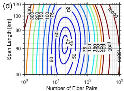
Figure 1: Trans-Pacific (11,000 km) link performance for the 125\mu\text{m}^2 , 0.155\text{ dB/km} fiber with PS-1 at 7 dB from Shannon Capacity (a) launch power per channel in dBm (b) spectral efficiency in bps/Hz (c) cable capacity in Tbps (d) normalized wet plant CPB.
