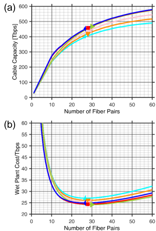
Figure 3: Advanced fibers compared to 80 \mu\text{m}^2 , 0.170 dB/km fiber over a 11,000 km Trans-Pacific link with PS-3 at 4 dB from Shannon Capacity (a) cable capacity (b) normalized wet plant cost per Tbps.
